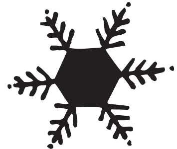
SNOWFLAKE # 6
