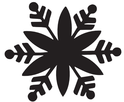
SNOWFLAKE # 9
