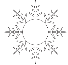
SNOWFLAKE # 3
