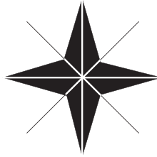
SNOWFLAKE # 2
