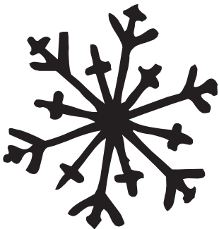
SNOWFLAKE # 7
