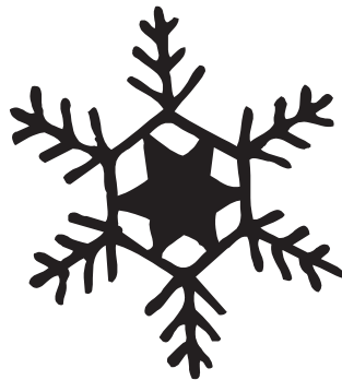
SNOWFLAKE # 8
