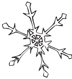
SNOWFLAKE # 5
