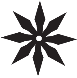
SNOWFLAKE # 1
