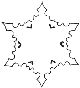
SNOWFLAKE # 4
